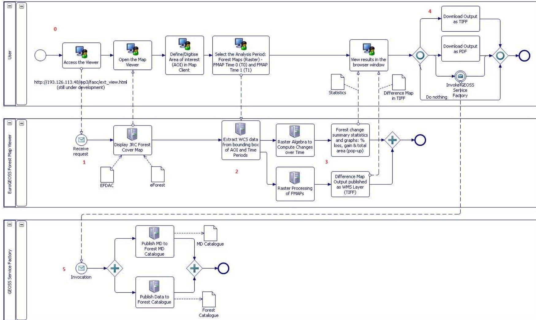
Figure 4: BPMN workflow of the forest change model (calculation of forest change i.e. loss/gain over a certain period)
