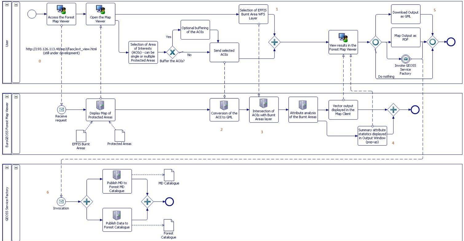
Figure 3: BPMN workflow of the forest fire model (calculation the bunt area within protected areas)
