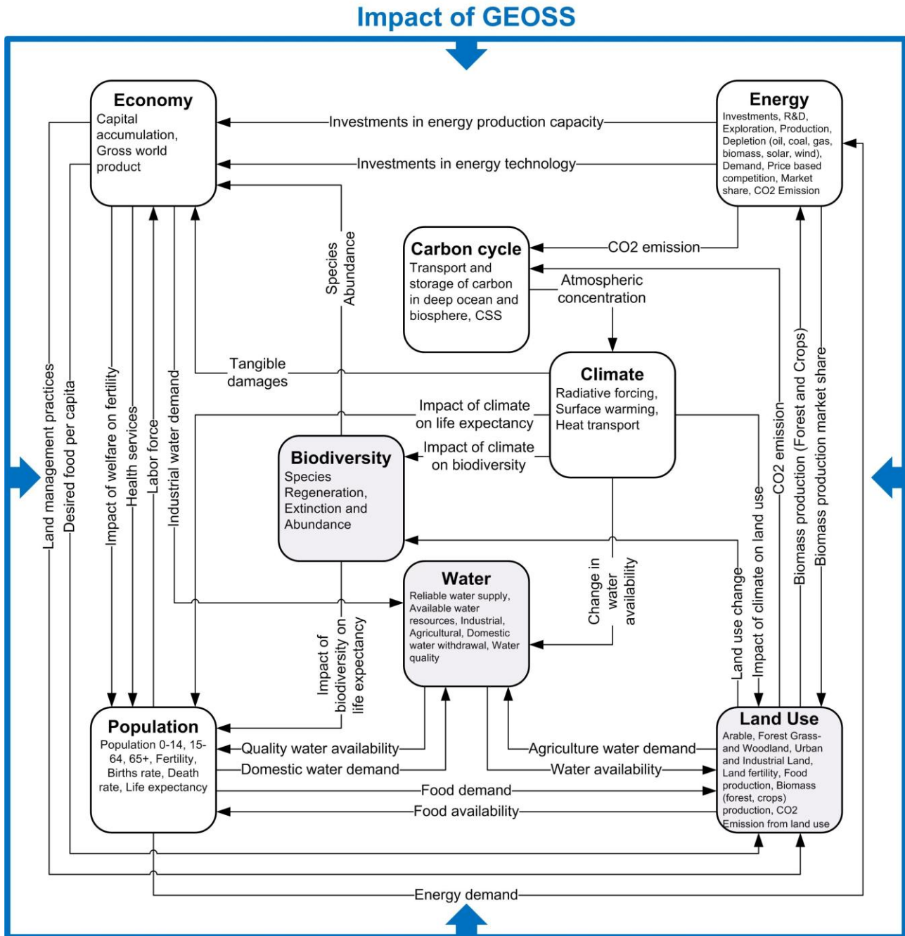
Figure 3: Overview of the FeliX model structure
